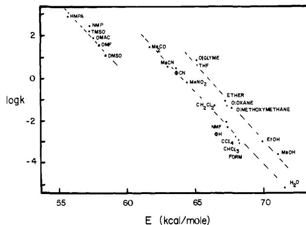
Figure 4. Plot of \log k values for the decarboxylation of 3-carboxy-6-nitrobenzoxazole (Table IIIA) as functions of the molar transition energy of the long wavelength electronic absorption maximum of the TMG salt of 2-cyano-5-nitrophenol.
