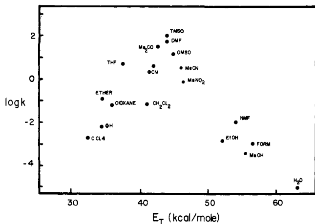
Figure 3. Plot of \log k values for the decarboxylation of 3-carboxy-6-nitrobenzoxazole (Table IIIA) as functions of the Dimroth E_T parameter.
